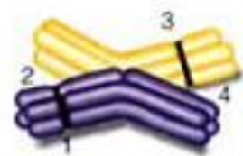
b Quadrivalent pairing during prophase I
