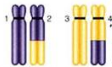
a Chromosomes in a reciprocal translocation heterozygote before chromosome pairing
