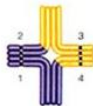
Early prophase I.
